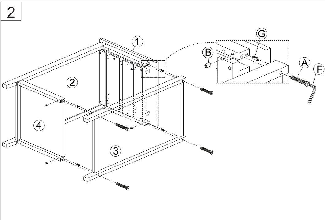
Image 2: Assemble the right side panel (3) and bottom panel (4) with top panel (1)
